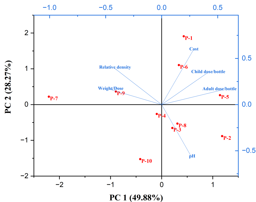
Fig. 6. Biplot illustrating the principal component analysis of the parameters.
