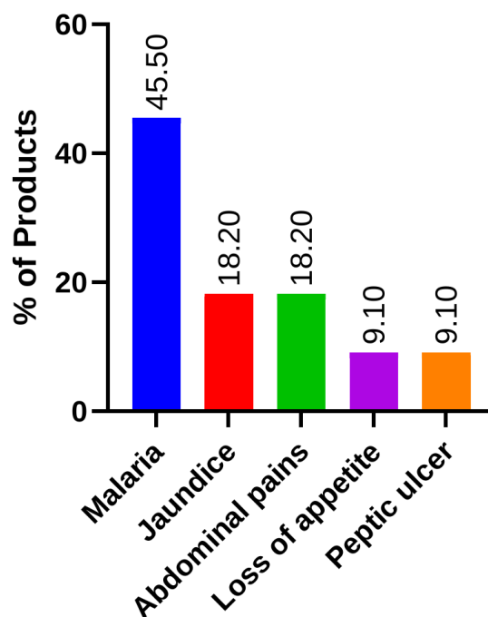
Fig. 2. Indications beyond typhoid listed on labels.
